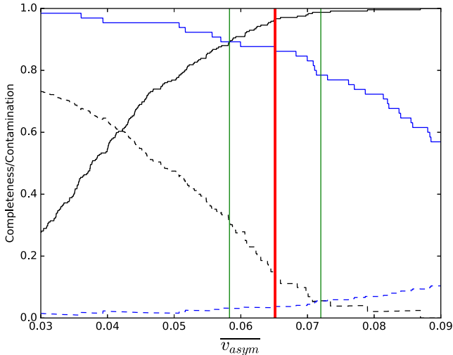
Figure 11. These curves show contamination (dashed) and completeness (solid) for visually asymmetric (blue) and visually normal (black) galaxies, at a range of values of \overline{v_{\text{asym}}} . We choose our cut-off point (shown in red) as the mid-point between the points of intersection of the curves for contamination (number of visually normal galaxies classified as kinematically asymmetric and vice versa) and completeness (number of visually asymmetric galaxies classified as kinematically asymmetric, similarly for visually normal galaxies) (shown in green). The points of intersection for contamination and completeness are 0.071 and 0.058, respectively, so we choose a cut-off value of \overline{v_{\text{asym}}} = 0.065 . See Section 4 for a complete explanation.
