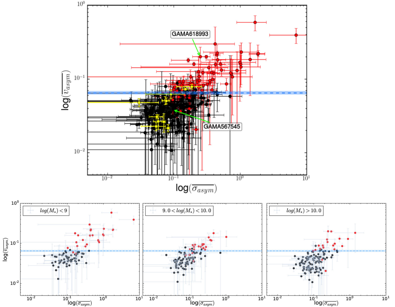
Figure 8. These plots summarize the results of kinematics for the 360 galaxies in our sample (top) and three stellar mass bins (bottom row). The median kinematic asymmetries for both velocity and velocity dispersion across fitted ellipse radii are normalized over the rotational velocity and plotted against each other. The sample was visually classified morphologically (using the SDSS DR10 images), with visually asymmetric galaxies shown here in red and ‘possibly asymmetric’ galaxies in yellow. We show the \bar{v}_{\text{asym}} cutoff for kinematic asymmetry derived in the text (blue, dashed line). The two example galaxies from Fig. 6, GAMA567545 (the normal galaxy) and GAMA618993 (the asymmetric galaxy) are indicated by the green arrows, for reference.
