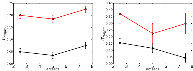
Figure 7. We show the values of v_{\text{asym}} (left) and \sigma_{\text{asym}} (right), with 1\sigma errors, at the positions of the semimajor radii of the fitted ellipses for an asymmetric (red, GAMA618993) and non-asymmetric (black, GAMA567545) galaxy. It can clearly be seen that the velocity and velocity dispersion asymmetry values for the asymmetric galaxy are significantly higher than those of the normal galaxy. These are the same two galaxies shown in Fig. 6.
