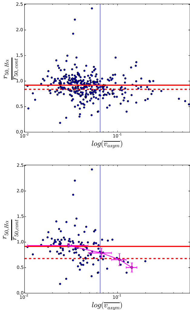
Figure 20. We show \log(\bar{v}_{\text{asym}}) against \frac{r_{50,\text{H}\alpha}}{r_{50,\text{cont}}} for all galaxies (top) and galaxies with \log(M_*) > 10.0 (bottom). The vertical blue line indicates the kinematic asymmetry cutoff \bar{v}_{\text{asym}} > 0.065 . Medians for normal (solid) and kinematically asymmetric (dashed) galaxies are shown in red. We see a 0.081 \pm 0.03 offset in median \frac{r_{50,\text{H}\alpha}}{r_{50,\text{cont}}} for all galaxies and 0.27 \pm 0.07 offset for high-mass galaxies, as well as an overall inverse correlation between \bar{v}_{\text{asym}} and \frac{r_{50,\text{H}\alpha}}{r_{50,\text{cont}}} in both cases. In the bottom panel, binned medians of \bar{v}_{\text{asym}} as a function of \frac{r_{50,\text{H}\alpha}}{r_{50,\text{cont}}} are shown in magenta, further demonstrating the downward trend. Vertical error bars show the error on the median and horizontal bars show the extend of the bins in \log(\bar{v}_{\text{asym}}) .
